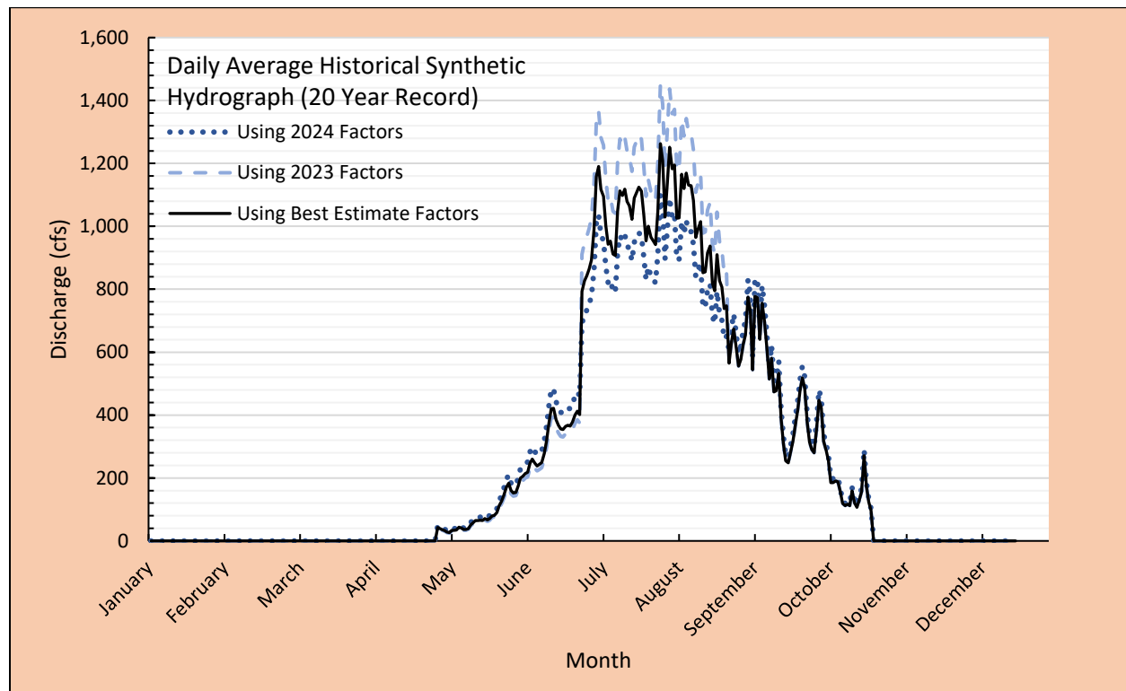
Figure 5: Average Historical Synthetic Hydrograph of the East Fork Martin River
